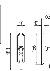
1422/M cremonese window lever handle
