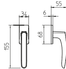
1872/DK martellina dk drehkipp system
