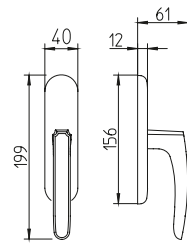
1872/M cremonese window lever handle
