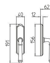
1342/M cremonese window lever handle
